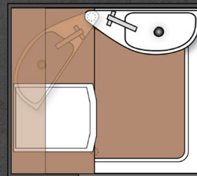
LAYOUT BIO dry separation toilet
