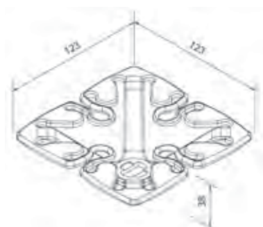
1 Federelement Spring element
