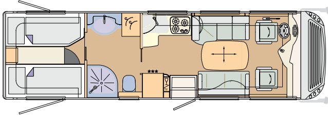
CHARISMA 840L LOUNGE Iveco Daily: 8480 x 2380 x 3290 mm, MAN: 8620 x 2380 x 3460 mm
