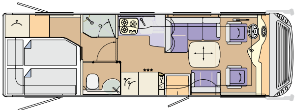
CHARISMA 791F Iveco Daily: 7980 x 2380 x 3290 mm, MAN: 8120 x 2380 x 3460 mm
