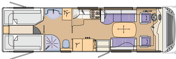
CHARISMA 890L LOUNGE Iveco Daily: 8980 x 2380 x 3290 mm, MAN: 9120 x 2380 x 3460 mm
