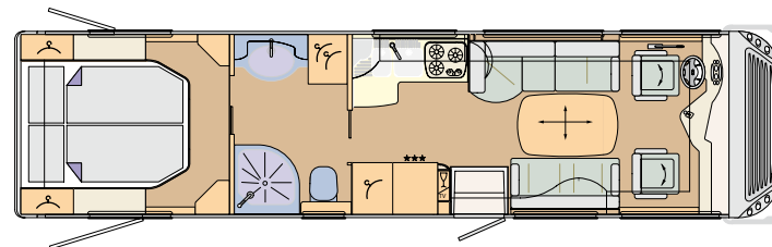
CHARISMA 940M LOUNGE Iveco Daily: 9480 x 2380 x 3290 mm, MAN: 9620 x 2380 x 3460 mm
