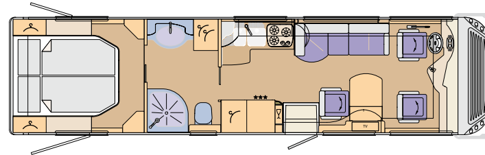
CHARISMA 940M Iveco Daily: 9480 x 2380 x 3290 mm, MAN: 9620 x 2380 x 3460 mm
