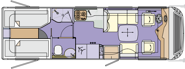
CHARISMA 791L Iveco Daily: 7980 x 2380 x 3290 mm, MAN: 8120 x 2380 x 3460 mm
