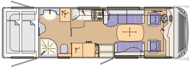
CHARISMA 840H LOUNGE Iveco Daily: 8480 x 2380 x 3290 mm, MAN: 8620 x 2380 x 3460 mm
