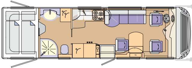
CHARISMA 840H Iveco Daily: 8480 x 2380 x 3290 mm, MAN: 8620 x 2380 x 3460 mm
