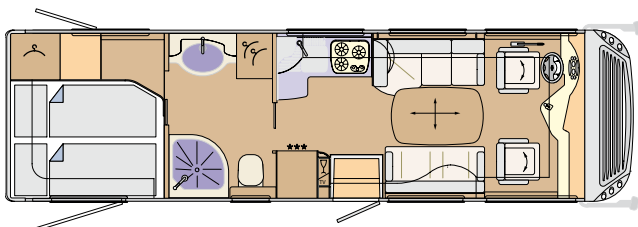
CHARISMA 840F LOUNGE Iveco Daily: 8480 x 2380 x 3290 mm, MAN: 8620 x 2380 x 3460 mm
