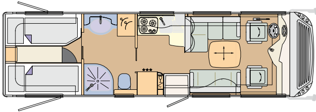
CHARISMA 840L C-LOUNGE Iveco Daily: 8480 x 2380 x 3290, MAN: 8620 x 2380 x 3460 mm
