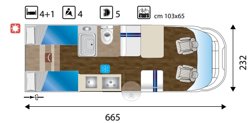
Therry 32
