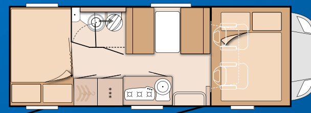
SKY TRAVELLER 650 DG SUPERLIGHT
