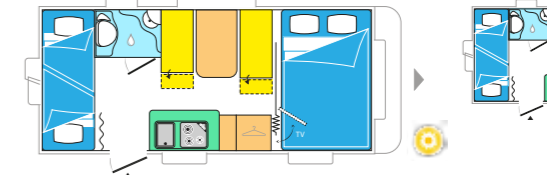
ANTARES 486 + PACK STYLE 486 FAMILY / 5,00 x 2,15 m
