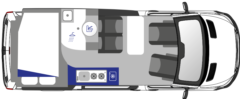
Day plan
