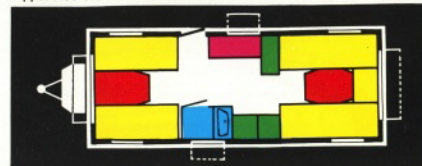
flipper-ASS 550 TS
