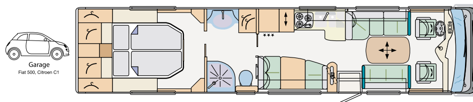
Liner 1130 Gmax Lounge
