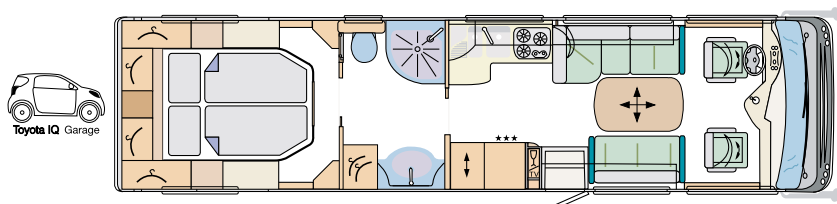
Liner 990 iQ Lounge
