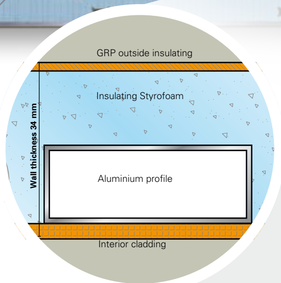
Aluminium profile
