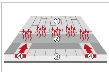
Floor temperature control system ALDE (optional, standard-equipped in the Scandica)
